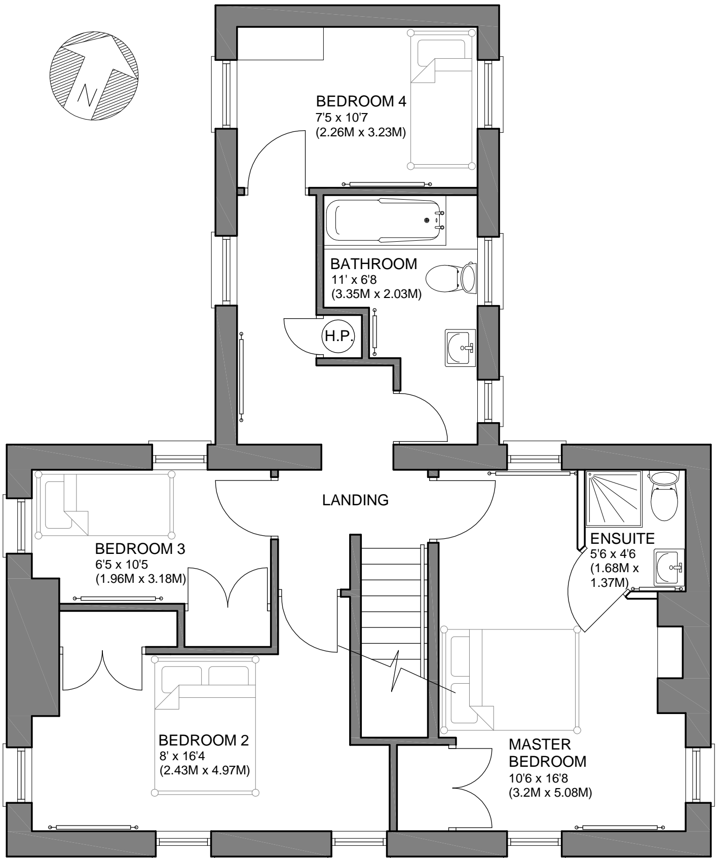
MUCHGRANGE - FIRST FLOOR PALN (AFTER RENOVATION WORKS)
