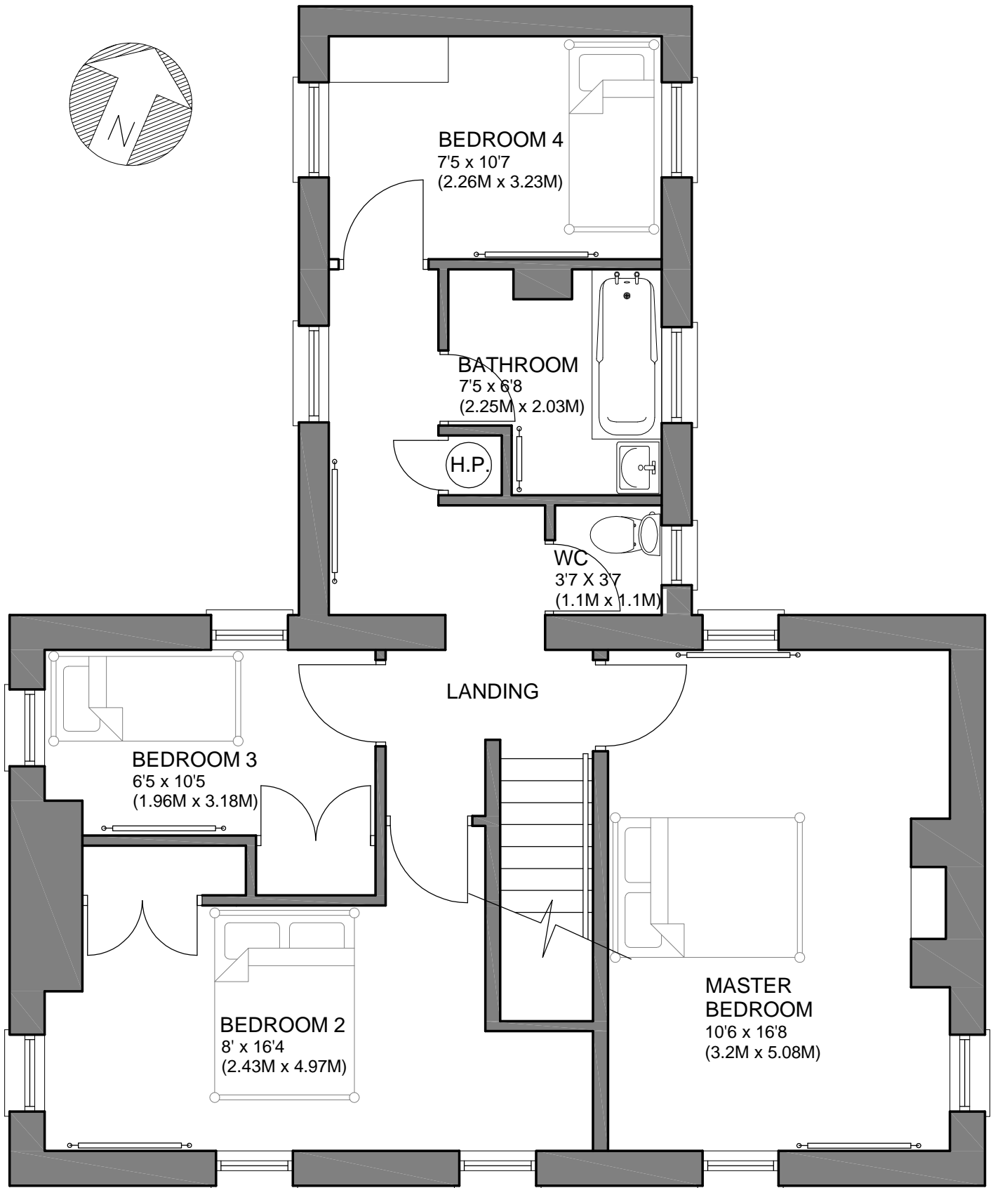
MUCHGRANGE - FIRST FLOOR PALN (BEFORE HOUSE FIRE)
