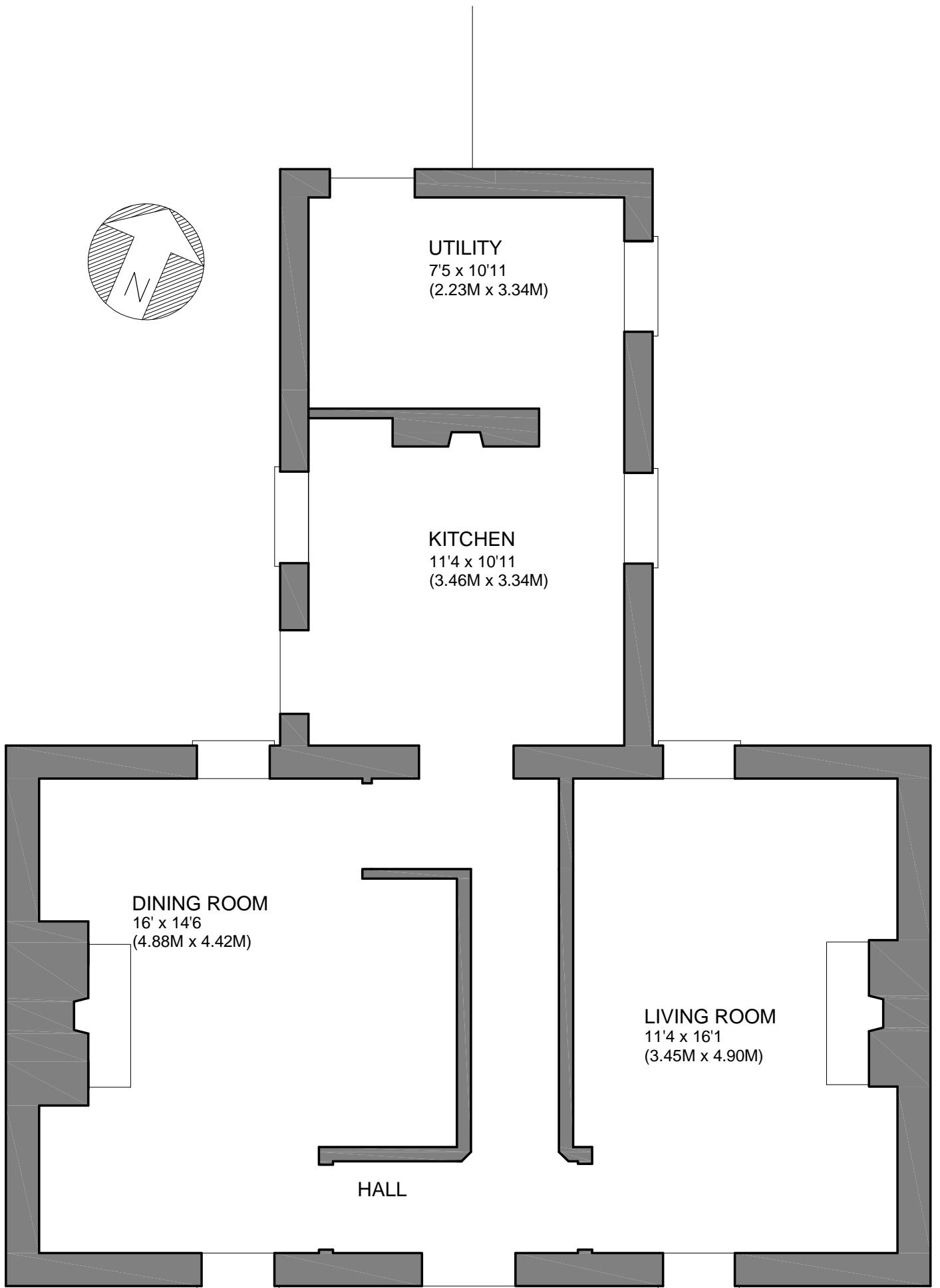
MUCHGRANGE - GROUND FLOOR PLAN (AFTER HOUSE FIRE AND BEFORE RENOVATION WORKS)
