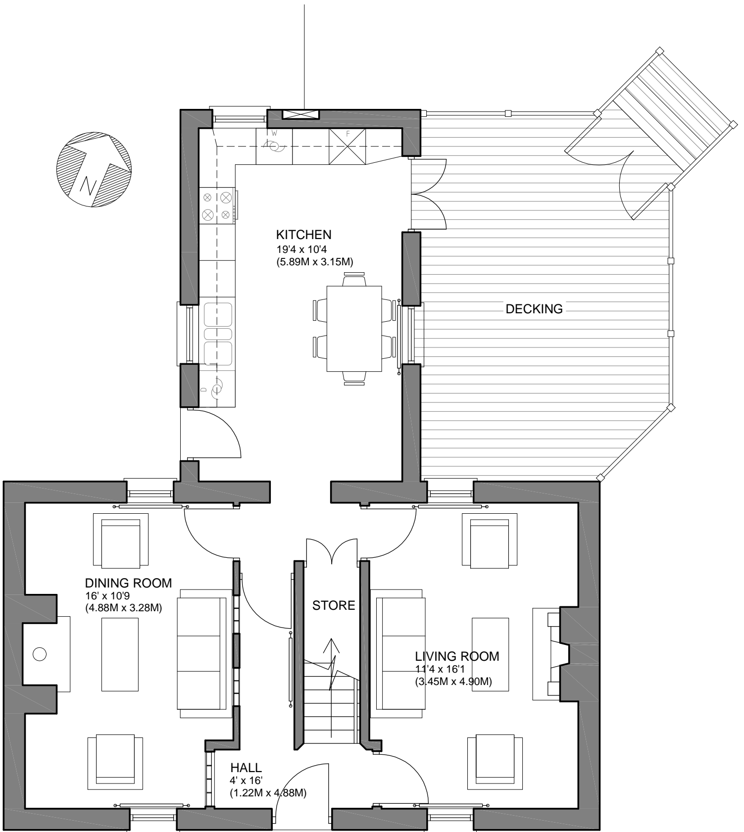
MUCHGRANGE - GROUND FLOOR PLAN (AFTER RENOVATION WORKS)
